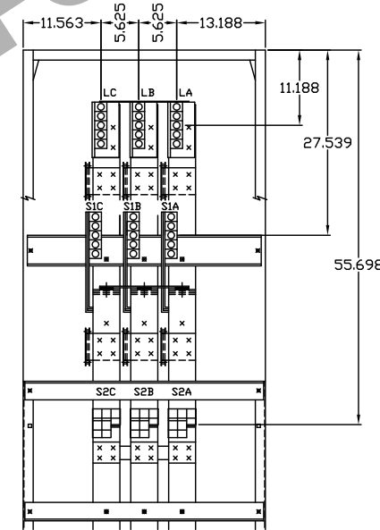
PARTIAL REAR VIEW SHOWING BUS MARKINGS
