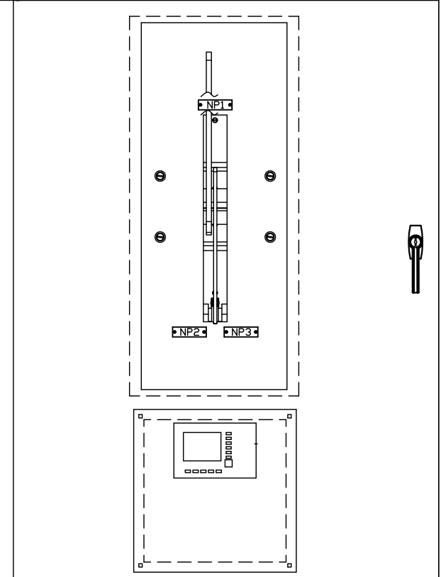
ENLARGED VIEW OF ACCESSORY PLATE AND SHIFTER PLATE (NAMEPLATE LOCATIONS)
