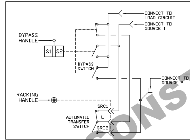
ONE LINE CONNECTION DIAGRAM
